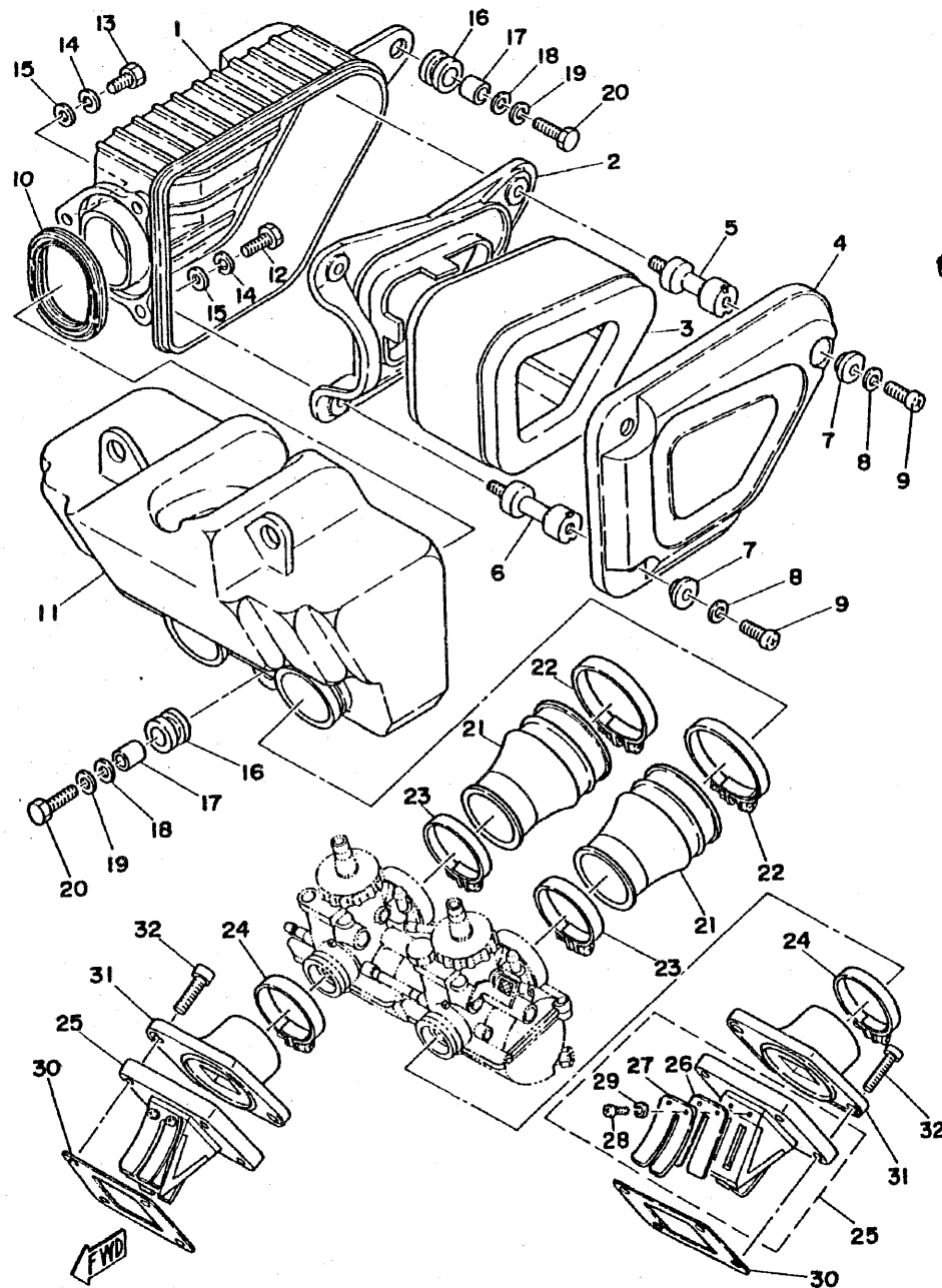
Fig. 10 INTAKE
