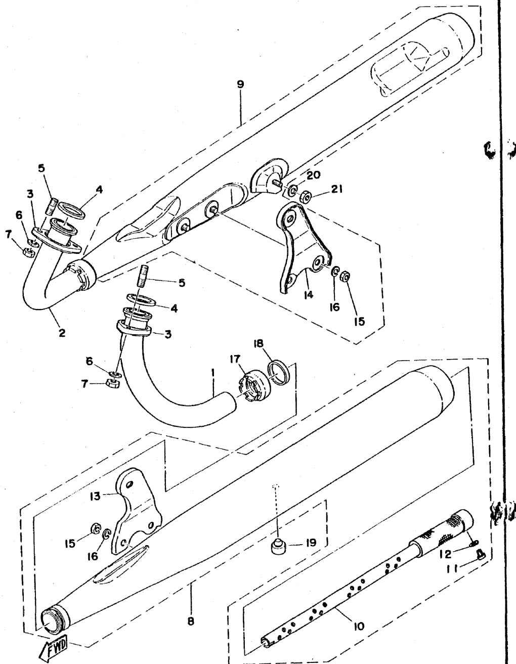
Fig. 12 EXHAUST
