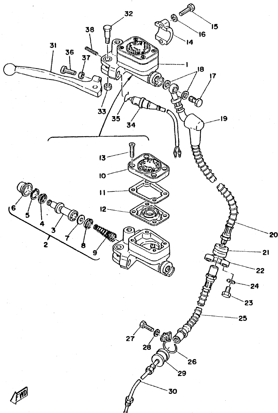
Fig. 23 MASTER CYLINDER · BRAKE HOSE
