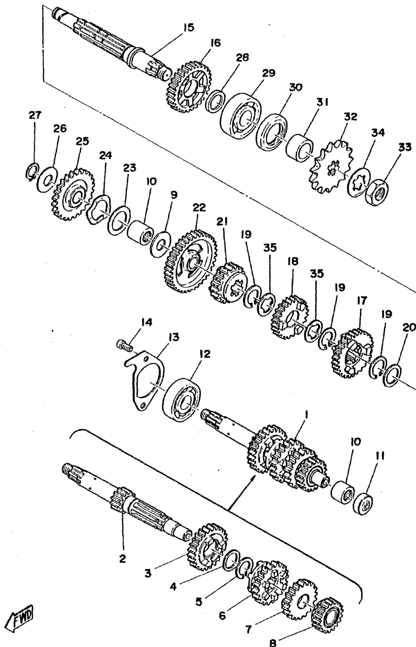
Fig. 5 TRANSMISSION
