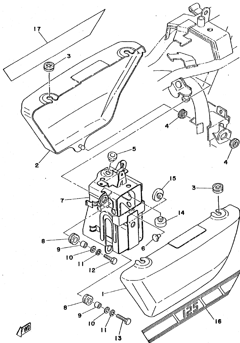
Fig.16 SIDE COVER · BOX
