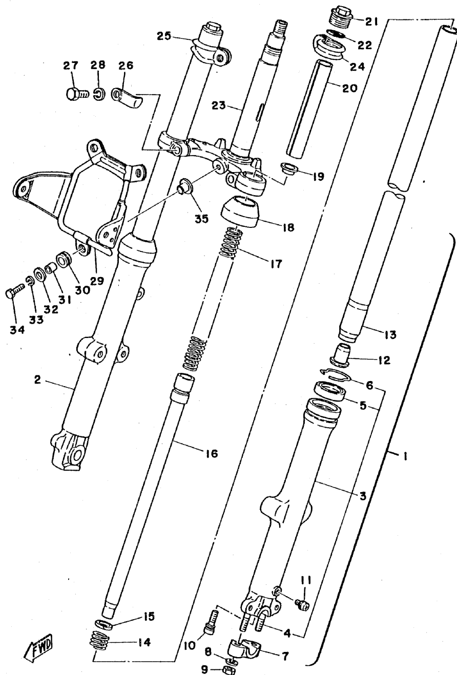
Fig. 20 FRONT FORK
