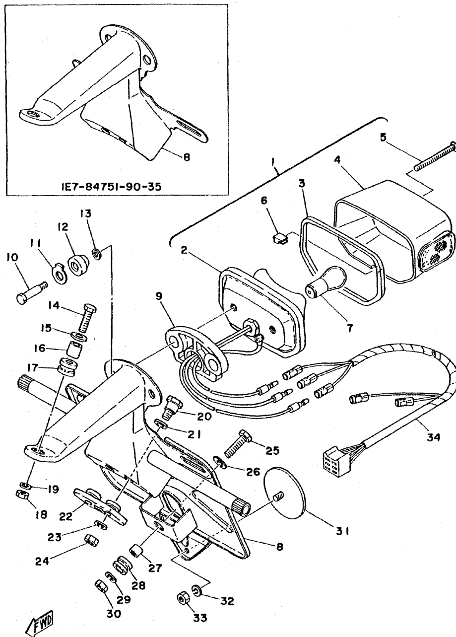
Fig. 33 TAIL LAMP 1
