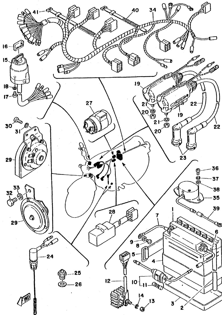
Fig. 37 ELECTRICAL
