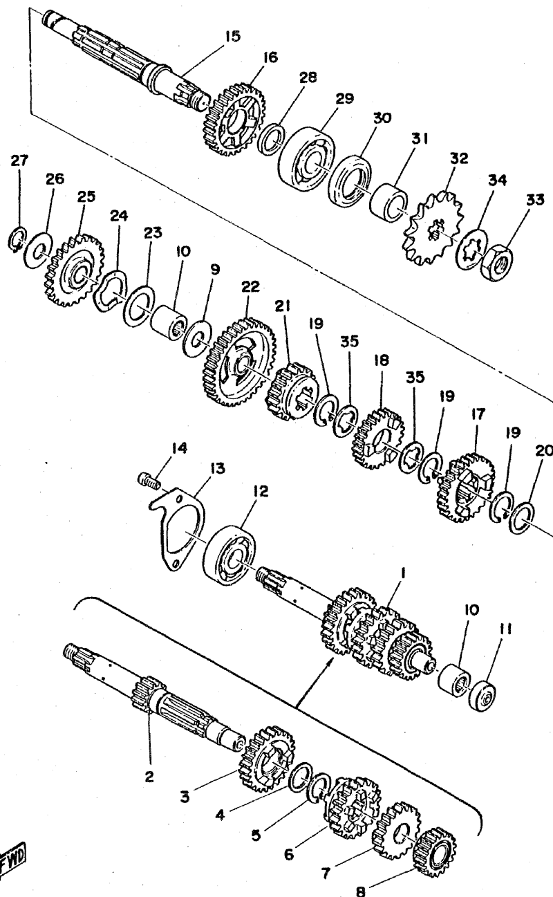
Fig. 5 TRANSMISSION
