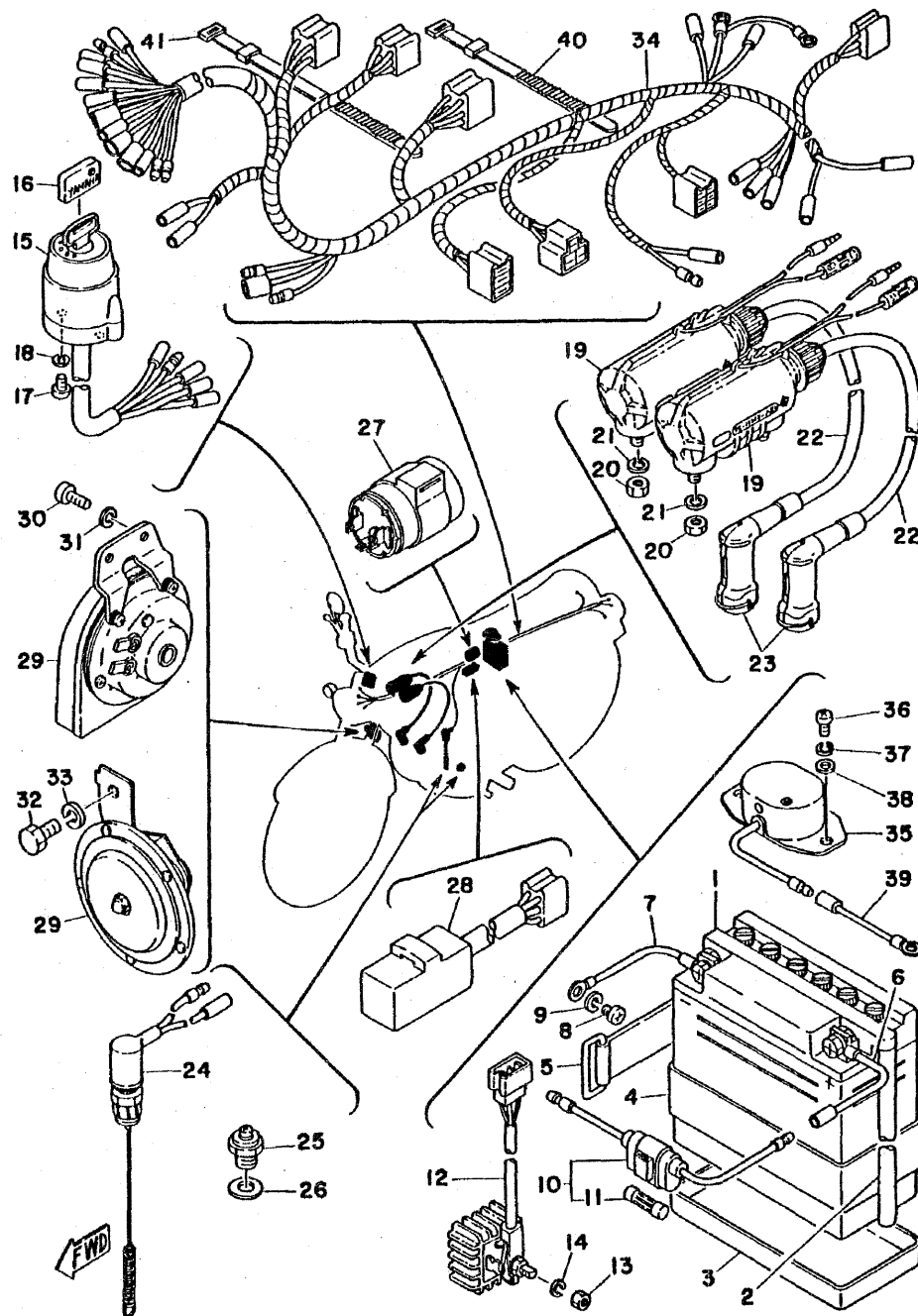
Fig. 37 ELECTRICAL
