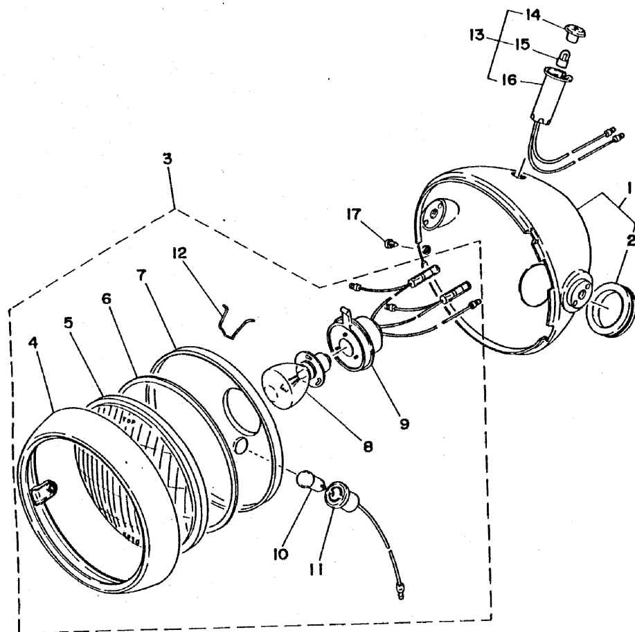
Fig. 31 HEAD LAMP 2
