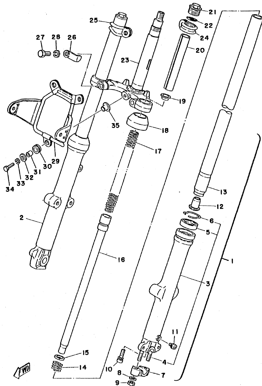
Fig. 20 FRONT FORK
