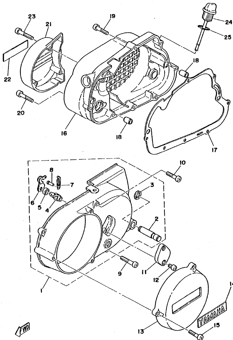
Fig. 2 CRANKCASE COVER
