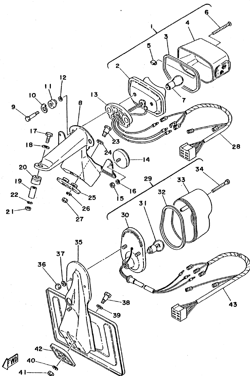
Fig. 34 TAIL LAMP 2
