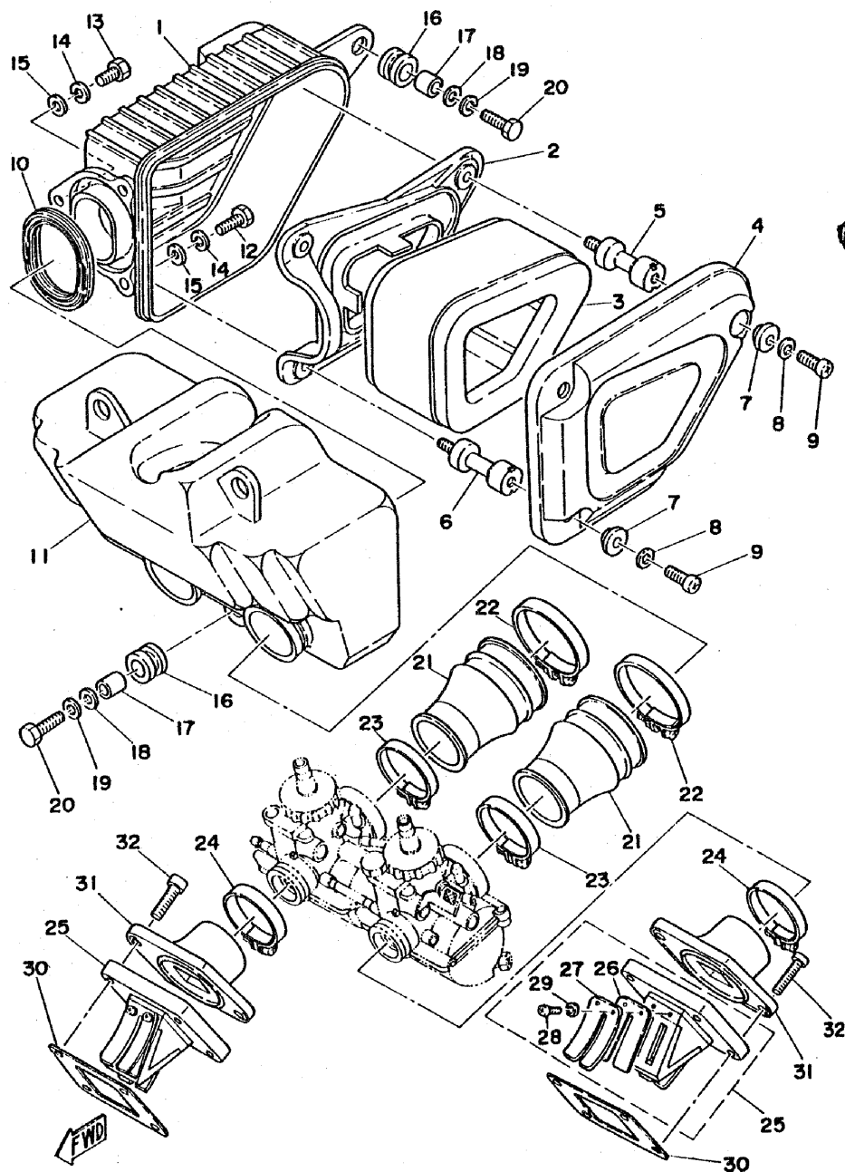
Fig. 10 INTAKE
