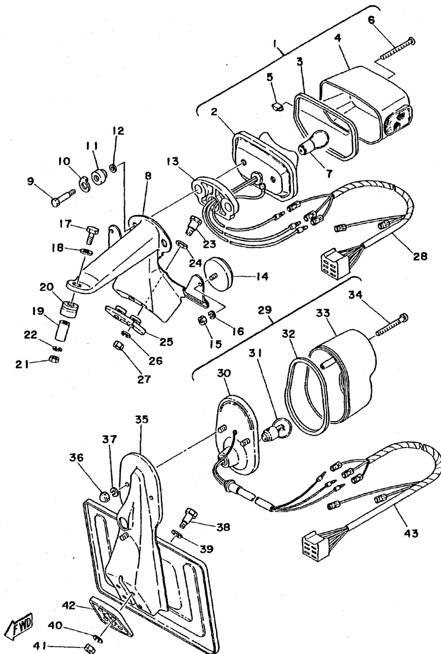
Fig. 34 TAIL LAMP 2
