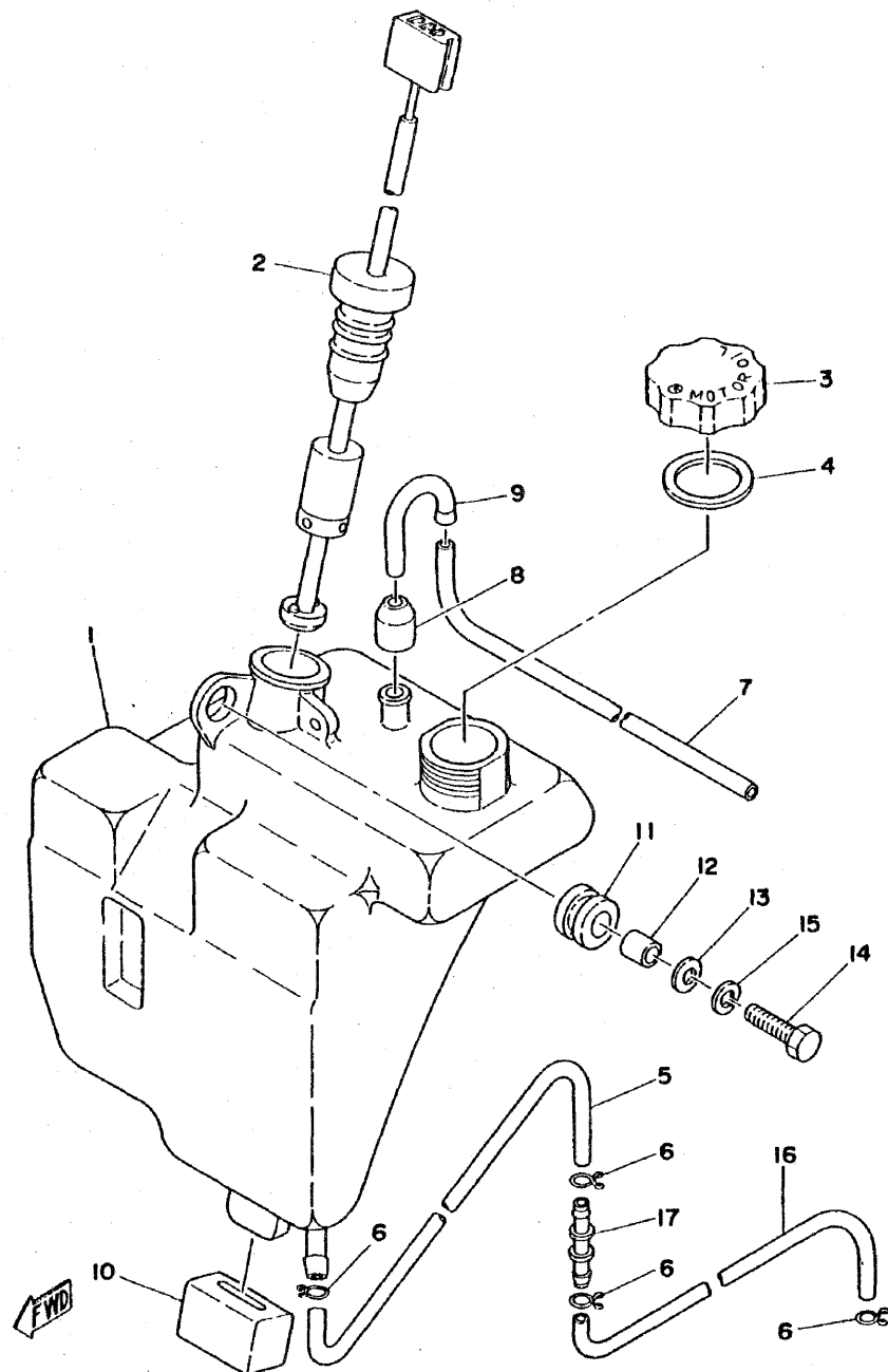
Fig. 25 OIL TANK
