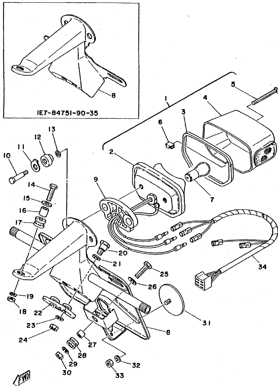
Fig. 33 TAIL LAMP 1
